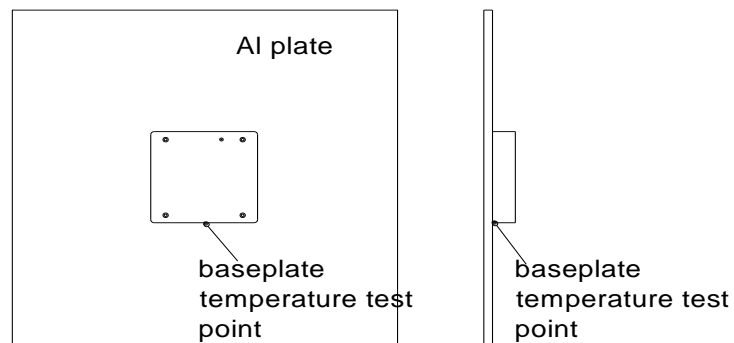
Figure 14: Temperature measured point
