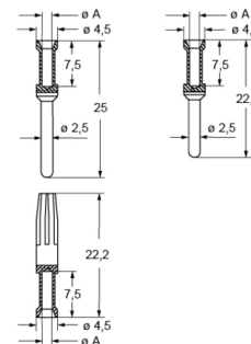
CCF, CCM and CC..AN contacts
